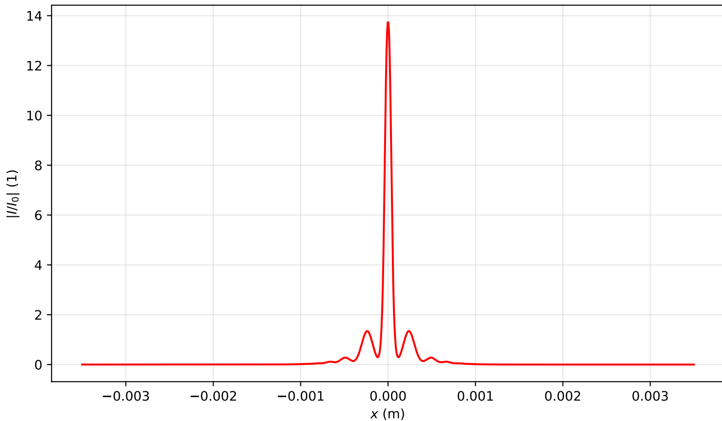
Intensity profile I(x, y = 0, z = 0.478)/I_0 , P_{in}=7.5P_{cr} , artificial time
